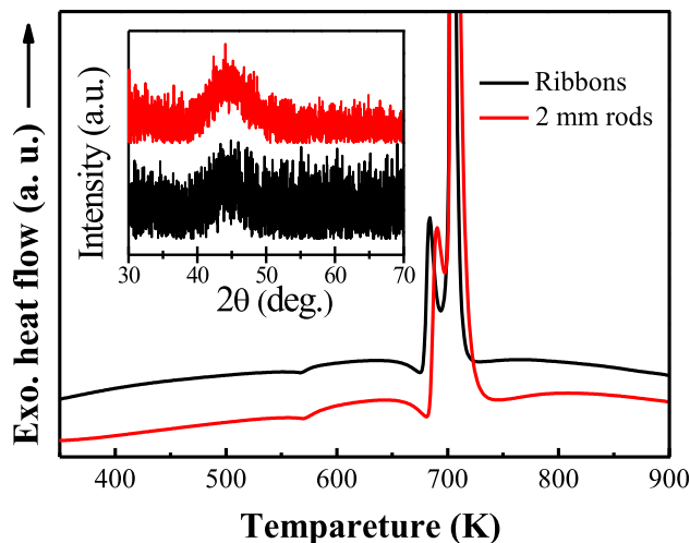
Fig. 1. XRD and DSC traces of as-cast \text{Fe}_{80}\text{P}_{13}\text{C}_7 glassy ribbons and rods.
